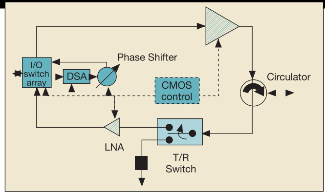
Figure 7. Phased Array Antenna Transmit/Receive T/R Control Block Diagram
