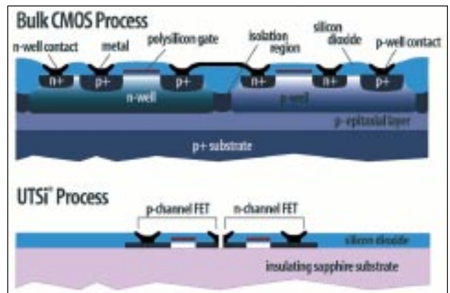
Figure 3. Cross Section of Bulk CMOS and UTSi CMOS Devices
