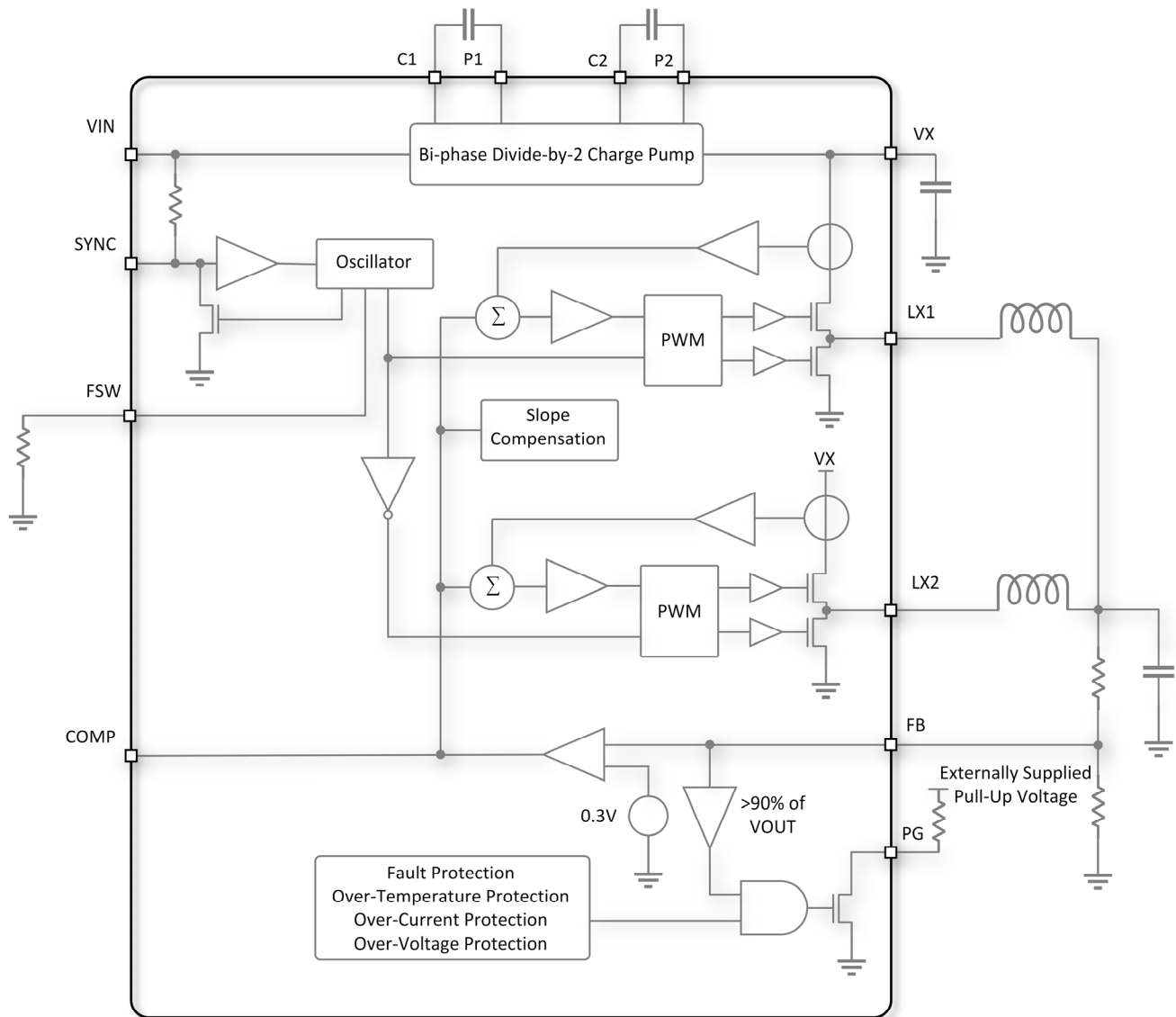
Figure 4. PE24111 Functional Block Diagram
