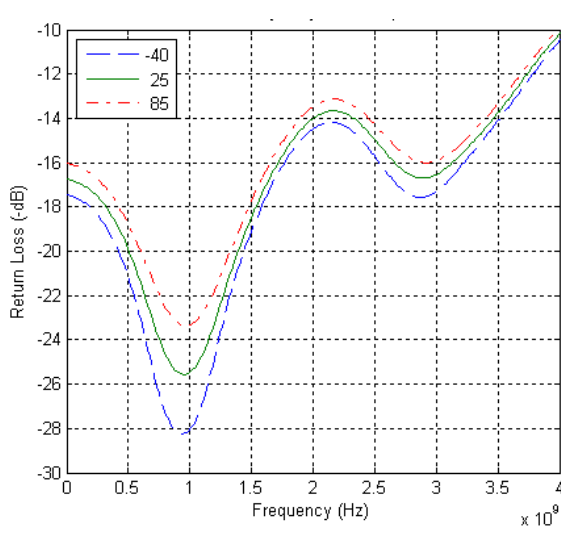
Figure 16. Return Loss: RFC @ 3.0 V
