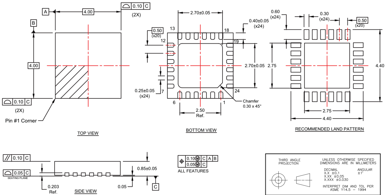
Figure 23 • Package Mechanical Drawing for 24-lead 4 x 4 x 0.85 mm QFN
