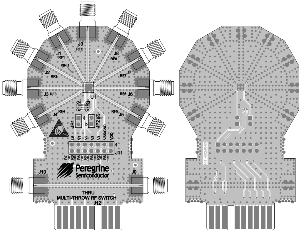
Figure 21 • Evaluation Board Layout for PE426482
