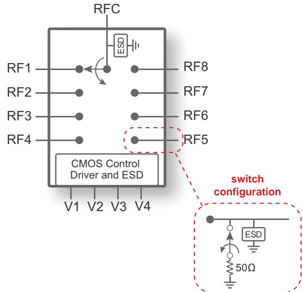
Figure 1 • PE426482 Functional Diagram
